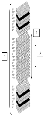
Figure 3: Lay-up of specimens.
